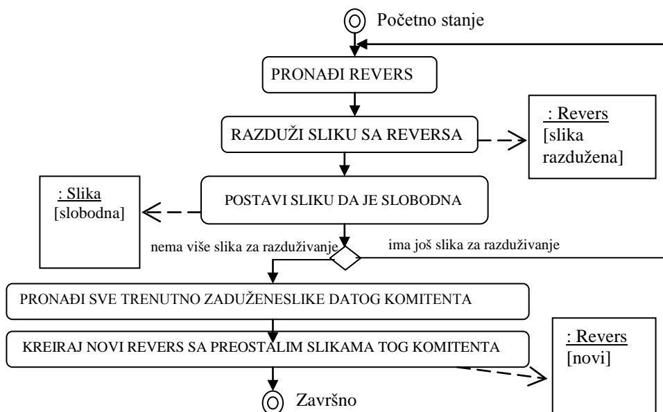
Slika 2.17. ACTIVITY DIAGRAM
