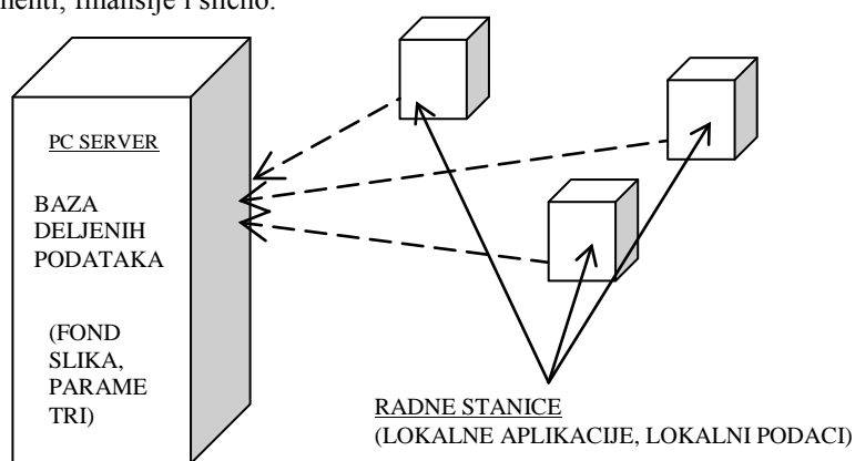
Slika 2.22. DEPLOYMENT DIAGRAM
