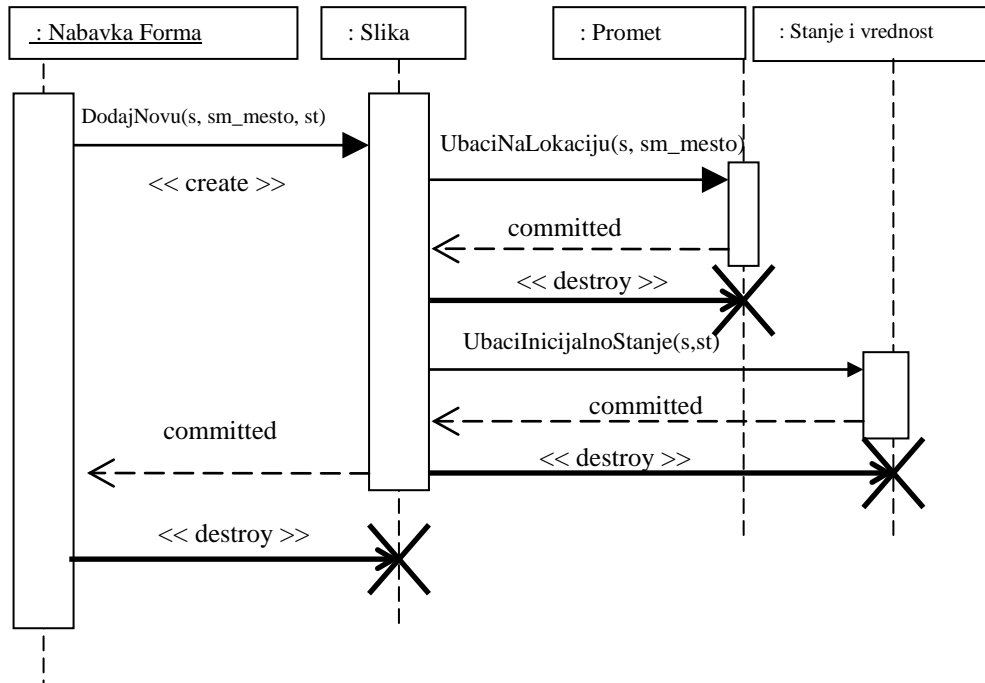
Slika 2.19. SEQUENCE DIAGRAM
