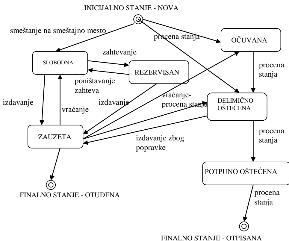
Slika 2.15. STATECHART DIAGRAM
