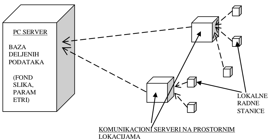
Slika 2.23. DEPLOYMENT DIAGRAM
