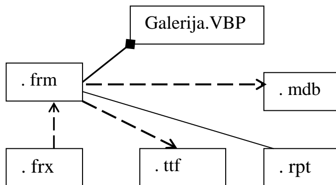
Slika 2.20. COMPONENT DIAGRAM
