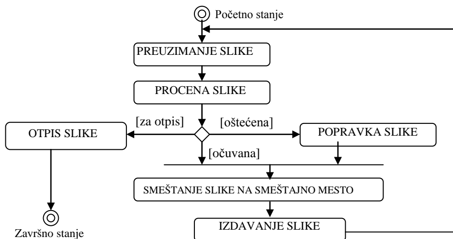
Slika 2.16. ACTIVITY DIAGRAM
