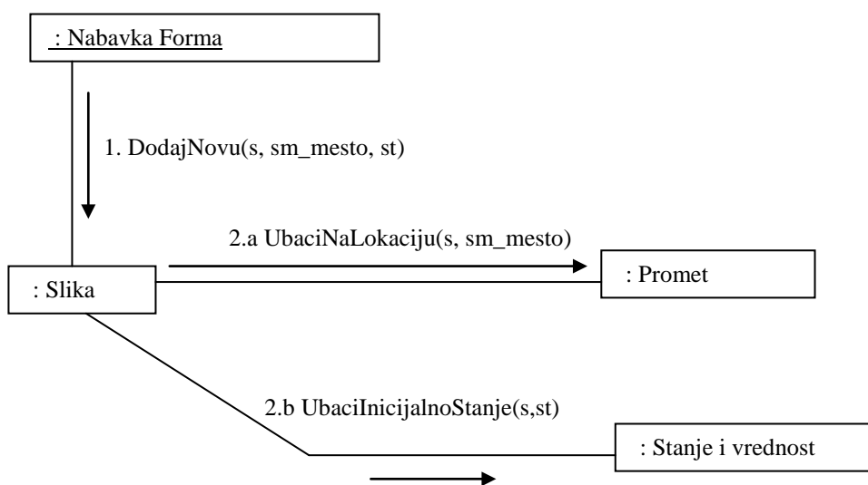
Slika 2.18. COLLABORATION diagram
